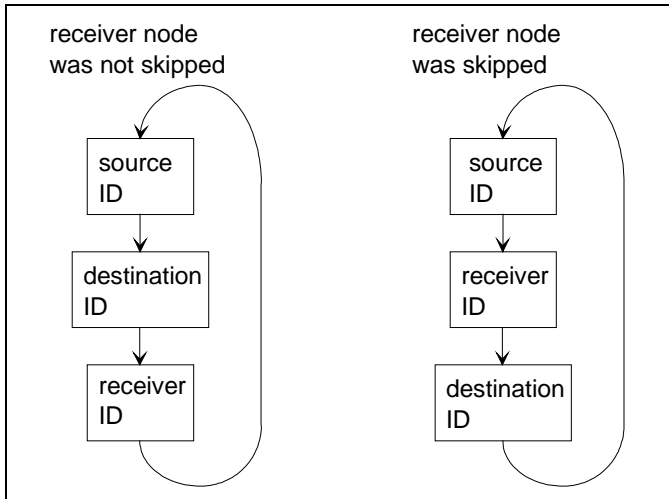
Figure 17 temporary logical ring for test, whether the receiver node has been skipped or not
