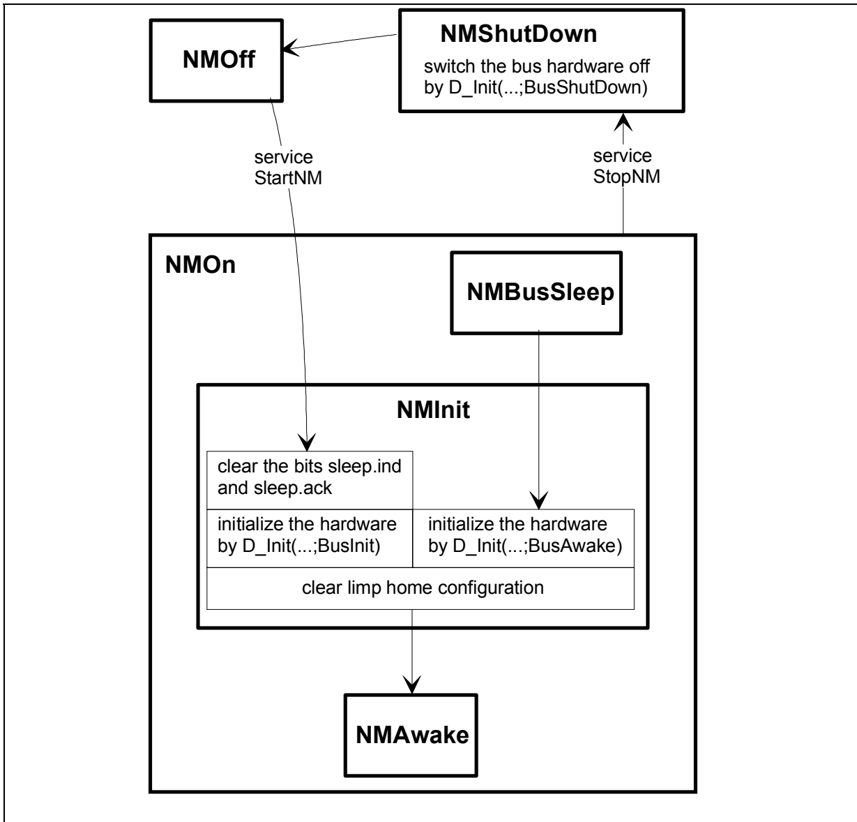
Figure 25 State transition diagram of NMIInit
