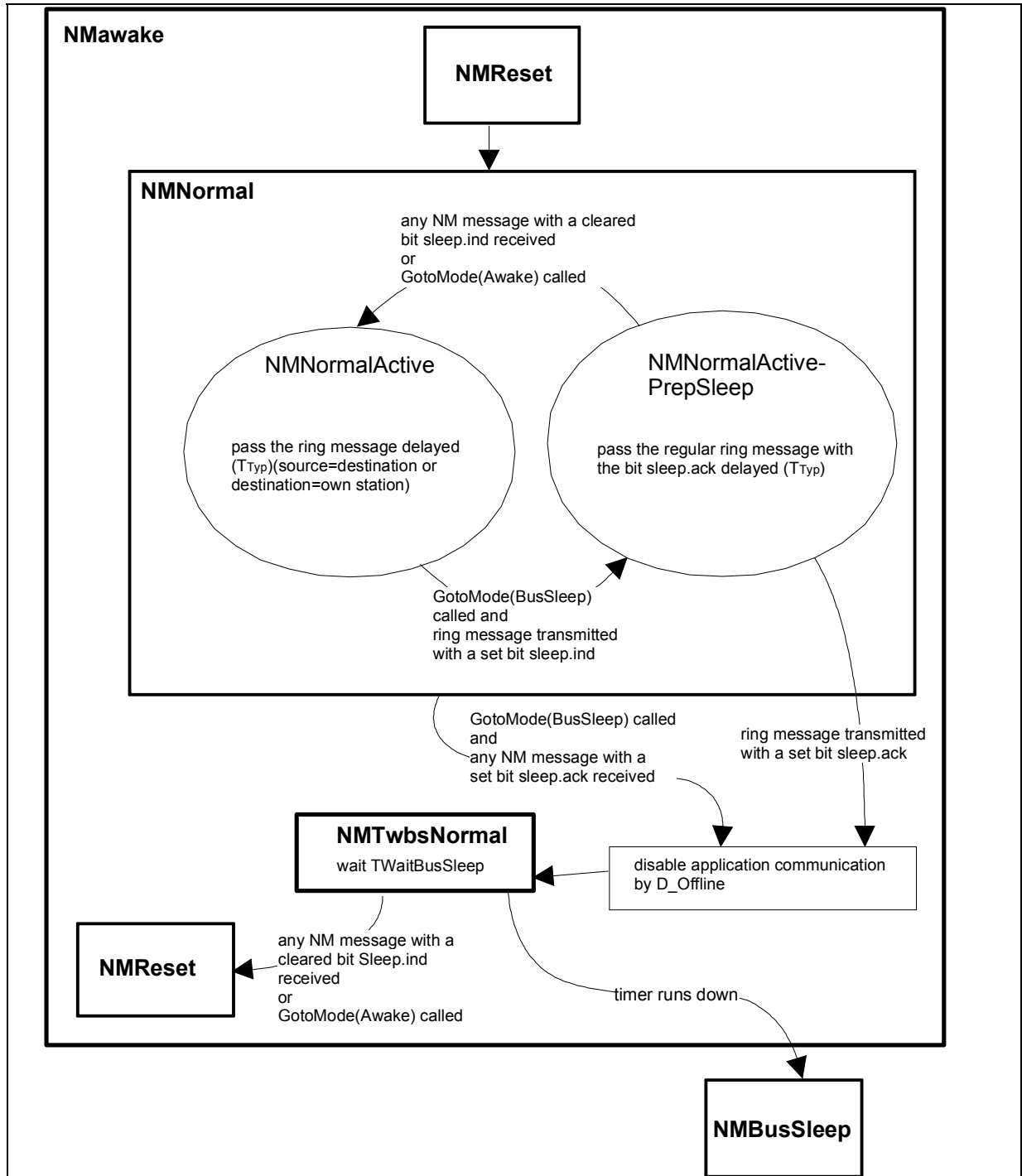
Figure 22 Algorithm for transition NMNormal → NMBusSleep
