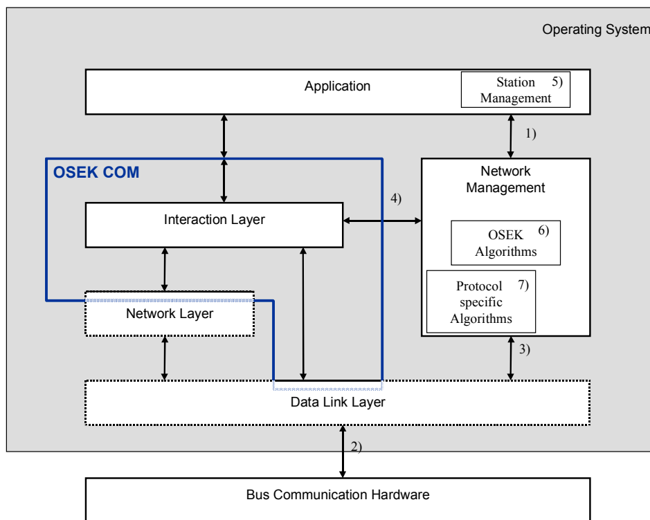
Figure 1 interface and algorithms responsibility 1) API, fixed by OSEK 2) several buses connected to one \mu Controller 3) interface to DLL - COM specific, protocol specific 4) interface to COM Interaction Layer 5) station management (outside OSEK, see text below) 6) OSEK algorithms 7) protocol specific management algorithms
