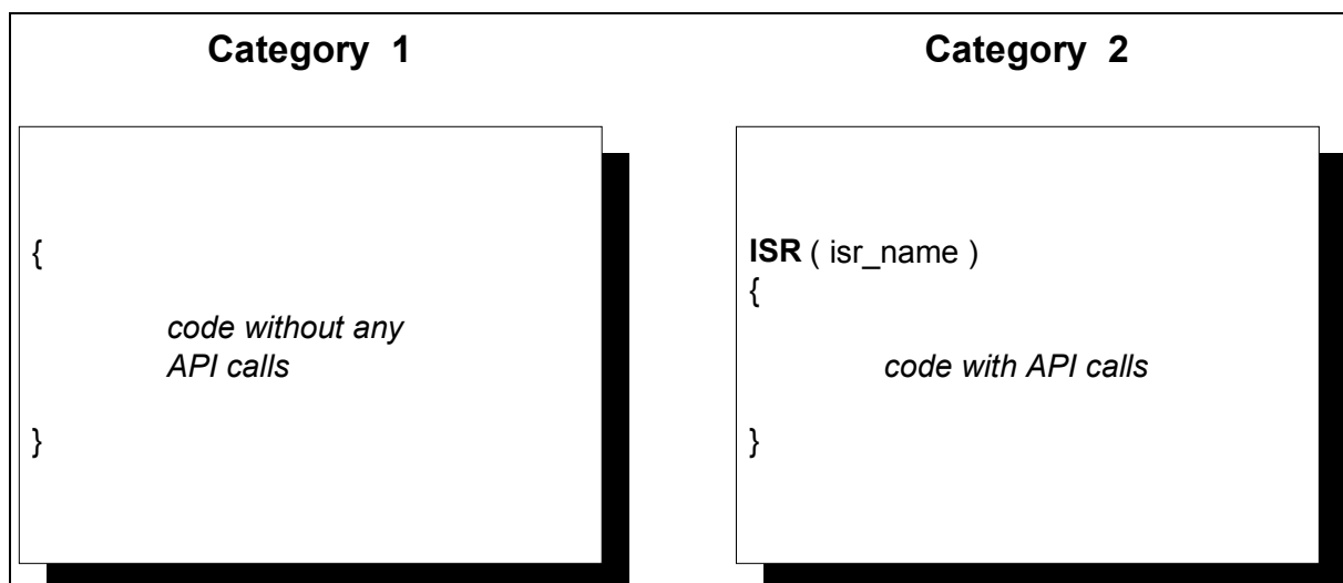
Figure 6-1 ISR categories of the OSEK operating system
