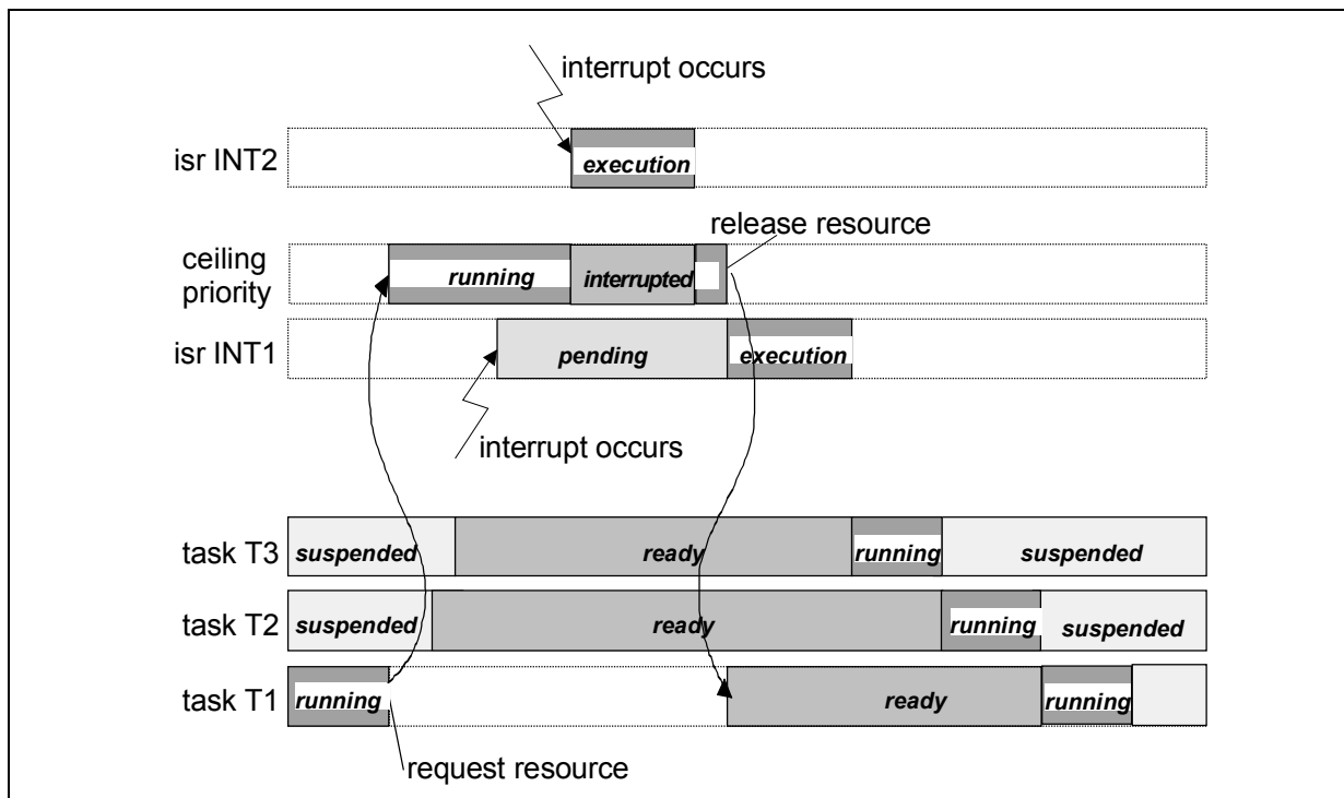
Figure 7-4 Resource assignment with priority ceiling between preemptable tasks and interrupt services routines.
