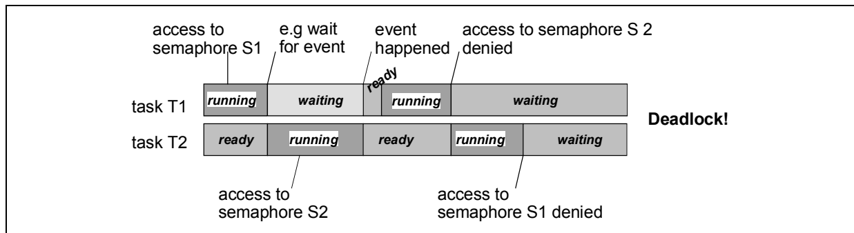
Figure 8-2 Deadlock situation using semaphores
