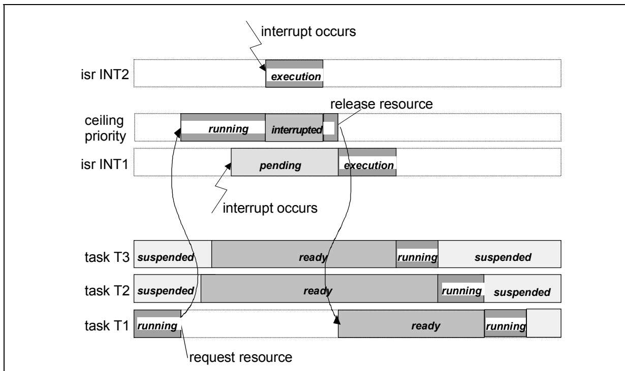
Figure 8-4 Resource assignment with priority ceiling between preemptable tasks and interrupt services routines.
